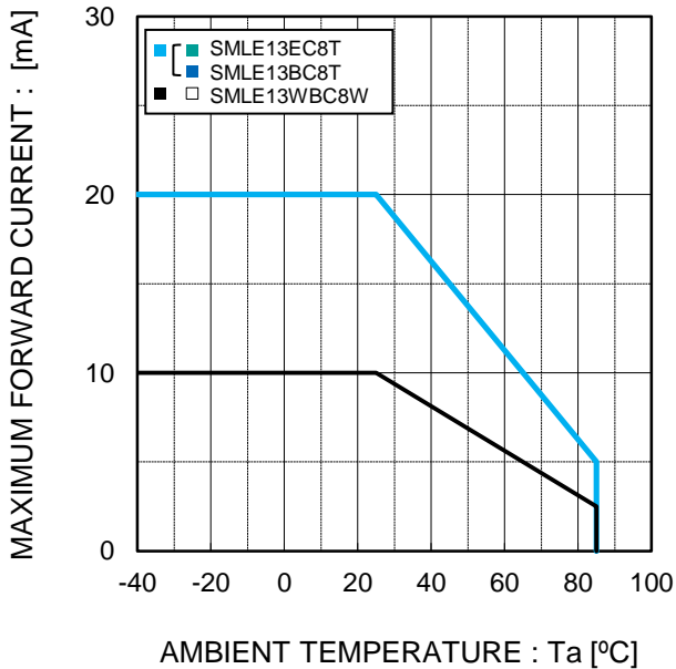
Fig.5 Derating
